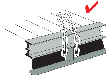
The chassis frame should be used as an anchorage point.
