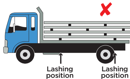
The dunnage is placed irregularly and could loosen or overtighten lashings when the vehicle is operating.
